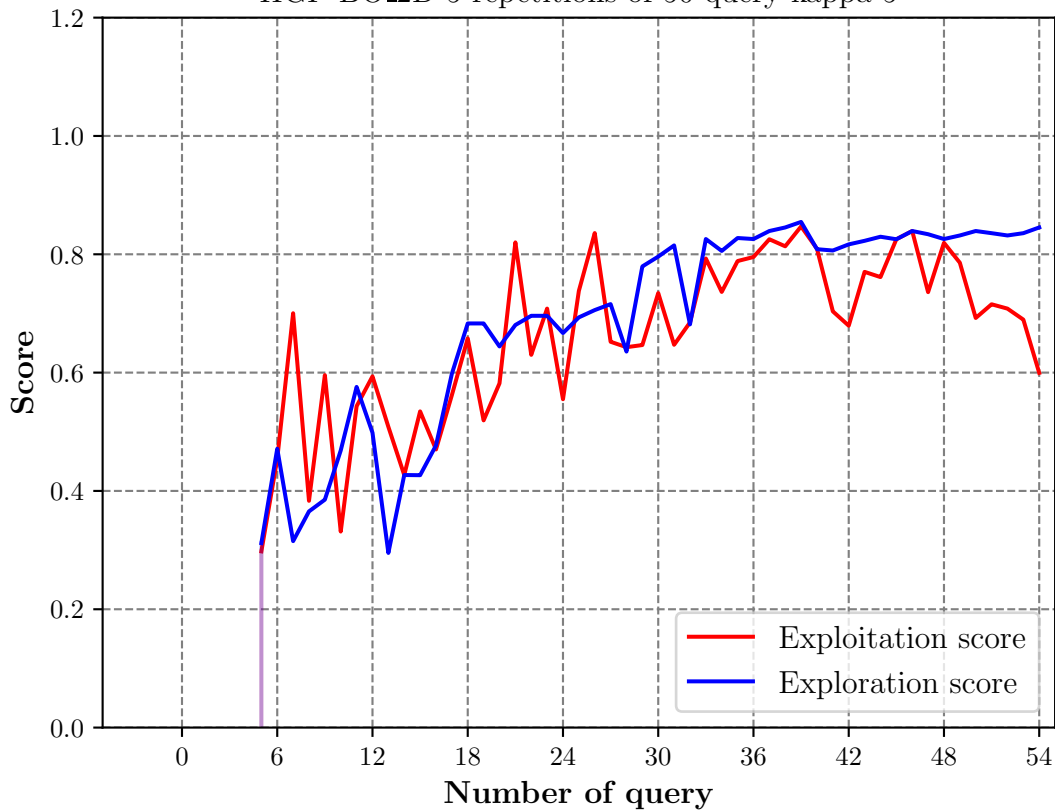
HGP-BO_2D 5 repetitions of 50 query kappa 5
